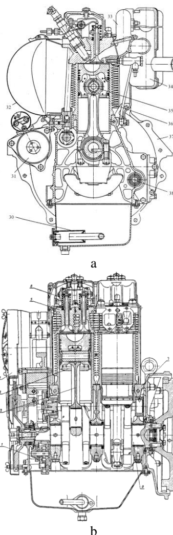
Figure 4 – Longitudinal section and cross-section of 2Ch10.85/12 diesel engine [39]
