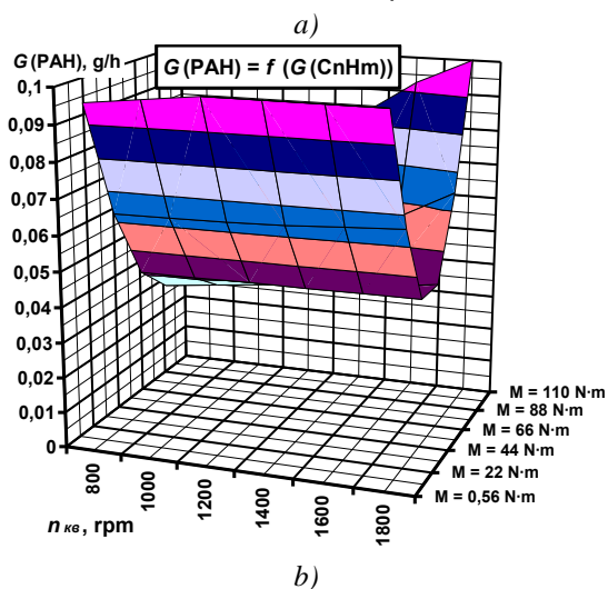
Fig. 2. Distributions of magnitudes of values G(B(a)P) = f(C_nH_m) (a) and G(PAH) = f(C_nH_m) (b) on operational modes field of 2Ch10.5/12 autotractor diesel engine [5]
