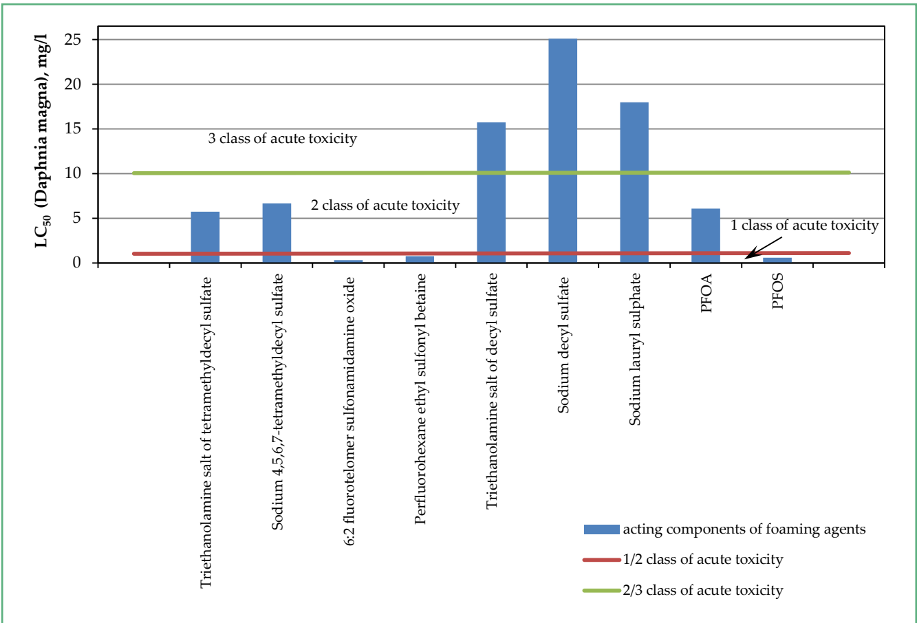
Fig. 11. The value of LC 50 (mg/l) on the effect of substances on Daphnia magna
