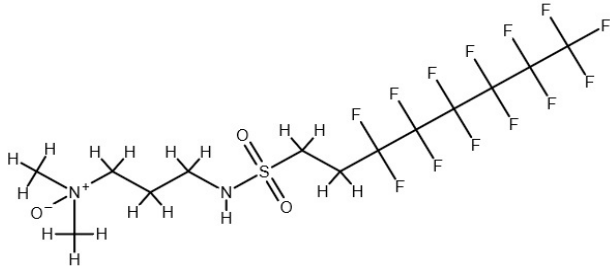
Fig.7. 2D structure 6:2 fluorotelomer sulfonamidamine oxide (N-[3-(dimethyl-oxo- \lambda^5 -azanyl)propyl]-3,3,4,4,5,5,6,6,7,7,8,8,8-tridecafluorooctane-1-sulfonamide)
