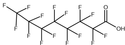
Fig.9. 2D structure PFOS
