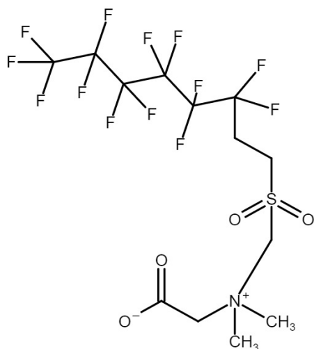
Fig.6. 2D structure Perfluorohexane ethyl sulfonyl betaine (2-{dimethyl[(3,3,4,4,5,5,6,7,7,8,8,8-tridecafluorooctanesulfonyl)methyl]azaniumyl}
