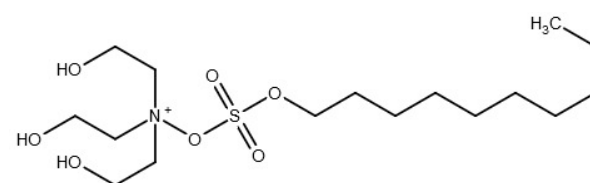
Fig.2. 2D structure Triethanolamine salt of decyl sulfate ([[decyloxy]sulfonyl]oxy)tris(2-hydroxyethyl)azanium)
