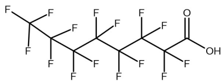
Fig.8. 2D structure PFOA
