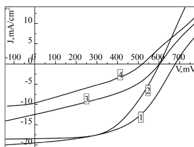
Fig. 1. Light CVCs of the solar cell: 1 – with a base layer thickness of 1 \mu\text{m} and irradiation from the front side; 2 – with a base layer thickness of 0.8 \mu\text{m} and irradiation from the front side; 3 – with a base layer thickness of 1 \mu\text{m} and radiation from the back side; 4 – with a base layer thickness of 0.8 \mu\text{m} and radiation from the back side
