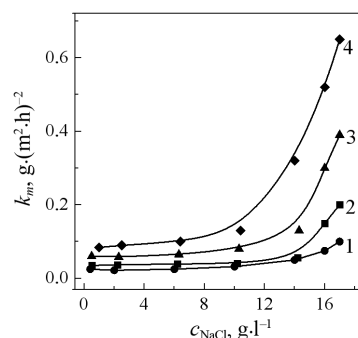
Fig. 1. Influence of NaCl concentration on corrosion rate of St. 3 steel and CI 18-36 cast iron in circulating water with pH=12 and temperature 22 °C: 1 – St. 3 in the volume of electrolyte; 2 – St. 3 in the waterline zone; 3 – CI 18-36 in the volume of the electrolyte; 4 – CI 18-36 in the waterline zone
