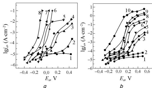
Fig. 3. Influence of pH value on the anodic polarization dependences: a – polarization dependences of steel St. 3 in water at pH=12. c(\text{NaCl}) , \text{g} \cdot \text{l}^{-1} : 1 – 0; 2 – 0.165; 3 – 0.195; 4 – 1.0; 5 – 1.65; 6 – 5.0; 7 – 6.6; 8 – 9.9; b – polarization dependences of cast iron CI 18-36 in water at pH=12. c_{\text{NaCl}} , \text{g} \cdot \text{l}^{-1} : 1 – 0; 2 – 0.165; 3 – 0.195; 4 – 1.0; 5 – 1.65; 6 – 5.0; 7 – 6.6; 8 – 9.9; 9 – 16.5; 10 – 20.0
