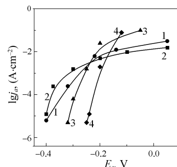
Fig. 2. Anodic polarization dependencies of CI 18-36 cast iron in water with pH=7. c_{\text{NaCl}} , \text{g} \cdot \text{l}^{-1} : 1 – 0; 2 – 5; 3 – 6.6; 4 – 10.0
