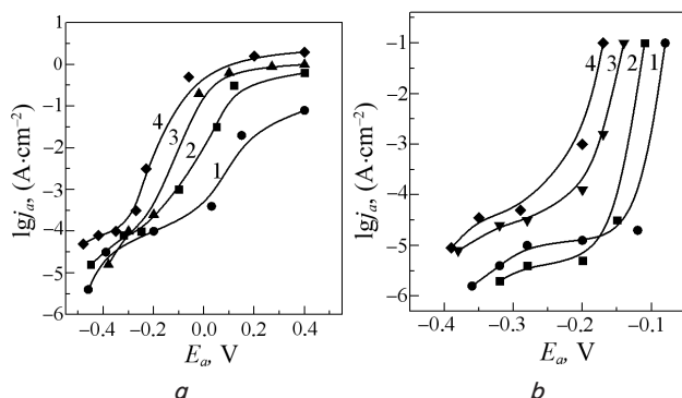
Fig. 4. Impact of water temperature on anodic polarization dependencies: a – polarization dependencies of steel St.3; t, °C: 20(1); 40(2); 50(3); 60(4). c NaCl =5,85 g·l -1 ; pH=12; b – polarization dependencies of cast iron CI 18-36; t, °C: 1 – 20; 2 – 40; 3 – 50; 4 – 60. c NaCl =5,85 g·l -1 ; pH=12
