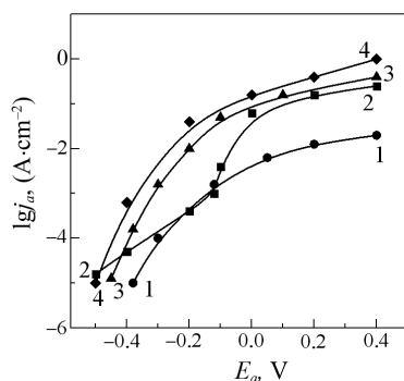
Fig. 5. Impact of water temperature on the anodic polarization dependencies of steel. t, ^\circ\text{C} : 1 – 20; 2 – 40; 3 – 50; 4 to 60. c_{\text{NaCl}} = 1,17 \text{ g}\cdot\text{l}^{-1} ; pH=7
