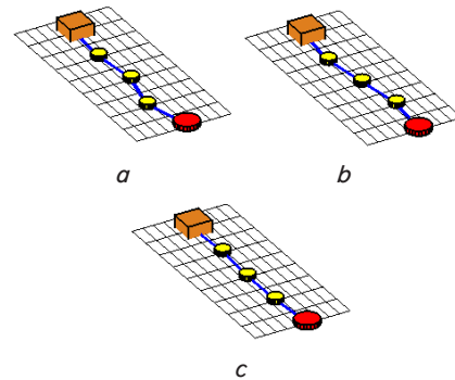
Fig. 5. Unfolding of pendulum links during final phases of oscillations: a - t=3.95; u_1=-0.1028; u_2=0.1619; u_3=-0.1965; u_4=0.2363; b - t=3.99; u_1=0.01216; u_2=0.006937; u_3=0.1984; u_4=-0.1183; c - t=4.02; u_1=-0.04290; u_2=0.1047; u_3=0.08769; u_4=-0.05071
