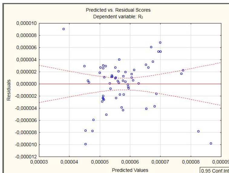
Fig. 7. The diagram of scattering the residuals from the predicted values
