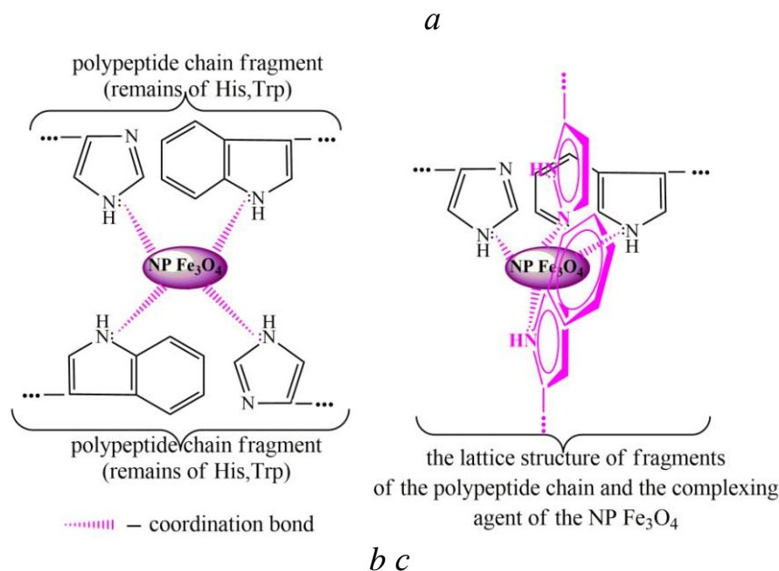
Fig. 6. Self-organization of the ligand and ferric iron ions of the Magnetofood nanoparticles into the lattice structure of the "cavitate" complex: self-organization of the ligand, fragments of two polypeptide chains and a complexing agent, ferric iron ions of the Magnetofood nanoparticles in a lattice structure ( a ); intermolecular complex, "cavitate" formed by the fragments of two polypeptide chains and the Magnetofood nanoparticles; spatial structure of "cavitate" formed by fragments of two polypeptide chains and \text{Fe}_3\text{O}_4 nanoparticles ( c )
