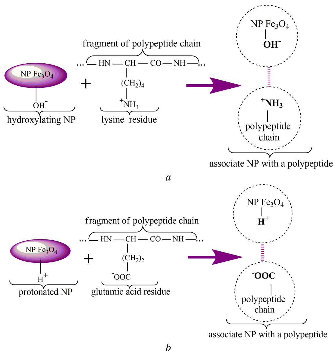
Fig. 2. Ionic interactions between ionized Magnetofood nanoparticles and charged ionogenic groups of polypeptides: hydroxylation of Magnetofood
